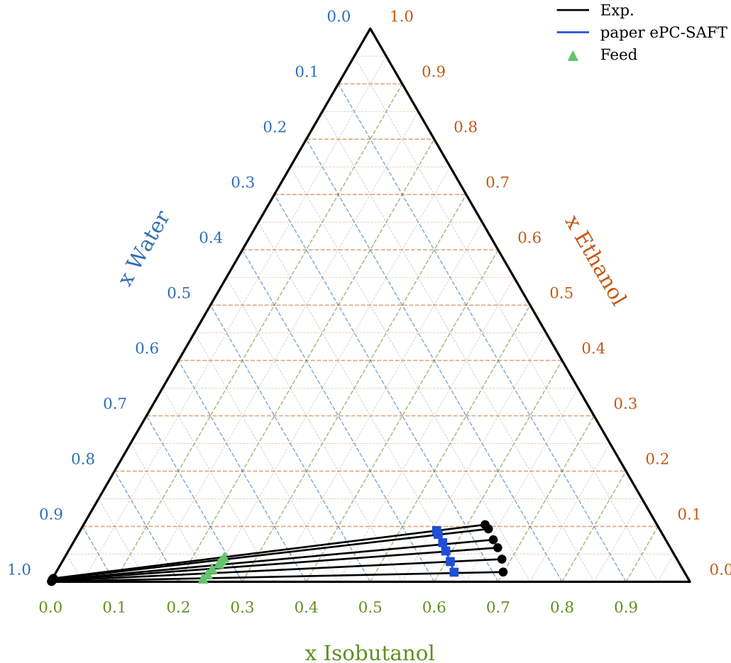
Figure 7. LLE for the system water + ethanol + isobutanol + 10 wt % NaCl at 313.15 K and atmospheric pressure expressed as salt-free composition: black (exp), package internal validation rejected all model tie-lines; no red model tie-lines are drawn, blue squares (paper ePC-SAFT organic branch, 6 points), and green (feed compositions).
