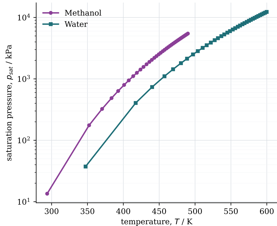
Water and methanol NIST saturation data
