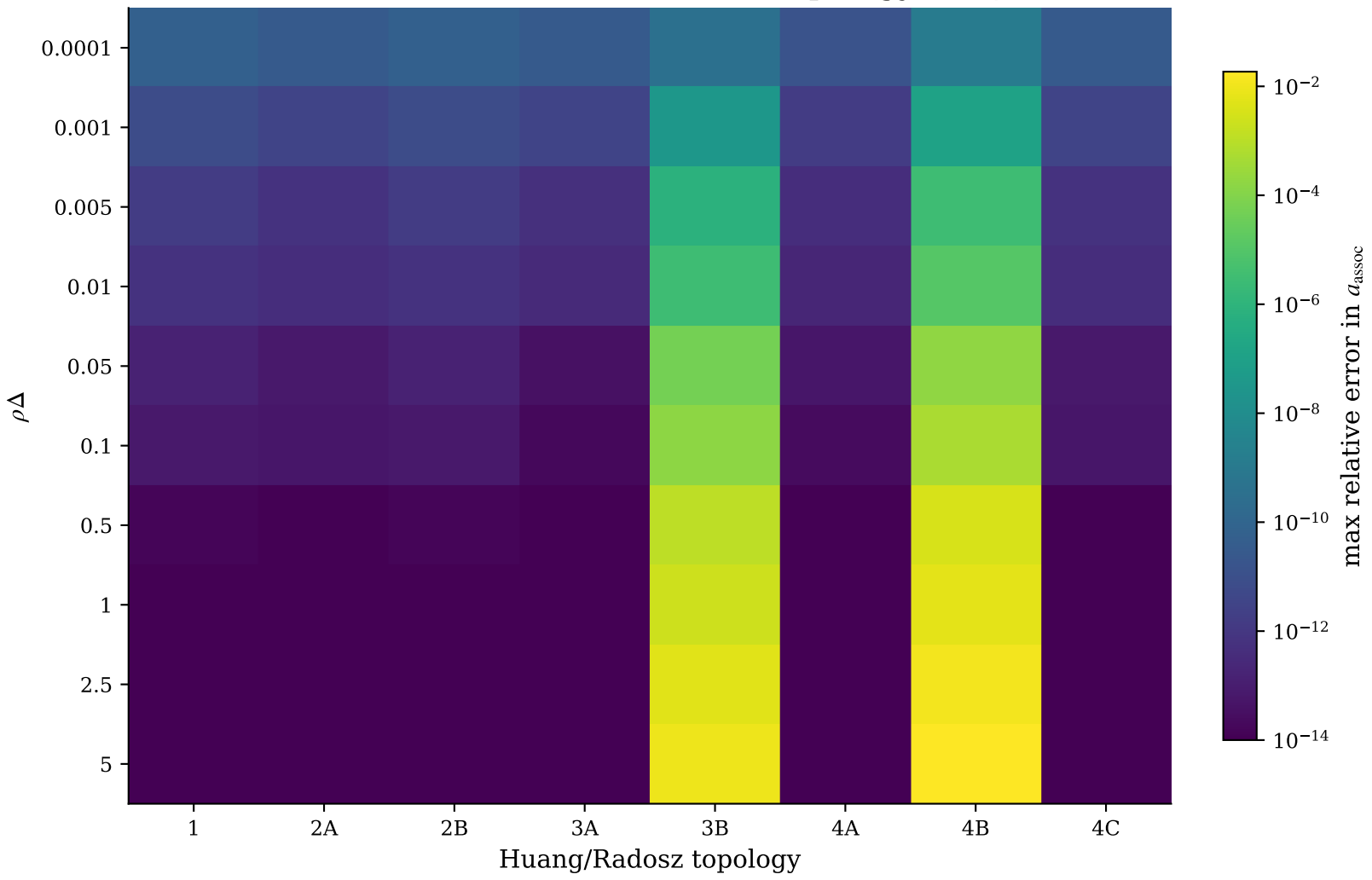
Picard association error across topology and \rho\Delta
