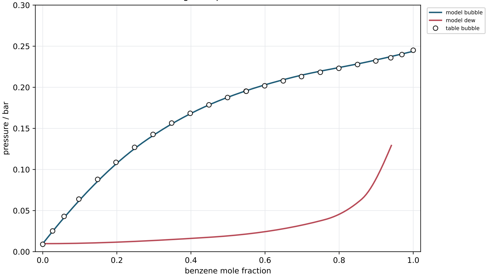
Gross 2002 Fig. 4: 1-pentanol/benzene at 40 C
