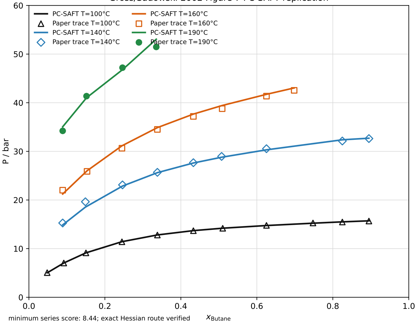
Gross/Sadowski 2002 Figure 7 PC-SAFT replication
