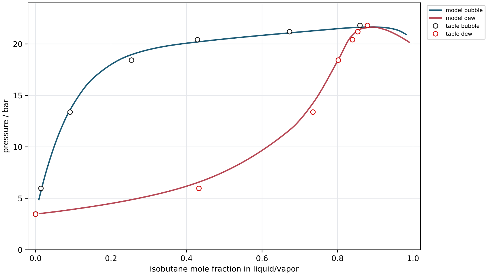
Gross 2002 Fig. 2: methanol/isobutane at 100 C
