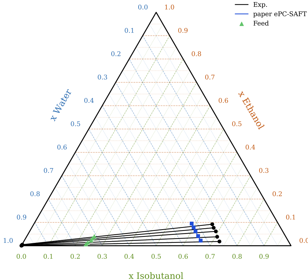
Figure 5. LLE for the system water + ethanol + isobutanol + 10 wt % NaCl at 293.15 K and atmospheric pressure expressed as salt-free composition: black (exp), package public ePC-SAFT rejected all model tie-lines; no red model tie-lines are drawn, blue squares (paper ePC-SAFT organic branch, 5 points), and green (feed compositions).
