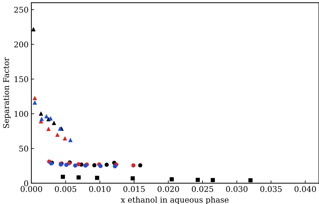
Figure 8. Separation factor of water over ethanol for the mixture water + ethanol + isobutanol + NaCl; black (293.15 K), red (303.15 K), blue (313.15 K), squares (without NaCl), circles (5 wt % NaCl), and triangles (10 wt % NaCl).
