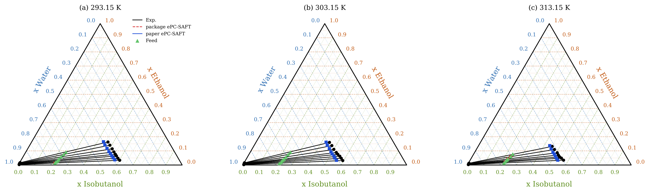
Figure S2. LLE for water + ethanol + isobutanol + 5 wt % NaCl at 293.15, 303.15, and 313.15 K: black (experimental), red dashed (package public electrolyte_ile solve), blue (paper ePC-SAFT), and green triangles (feed compositions).
