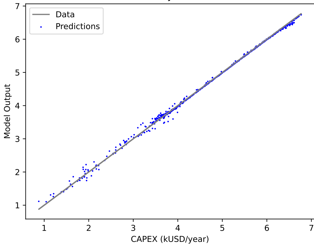
Parity Plot
