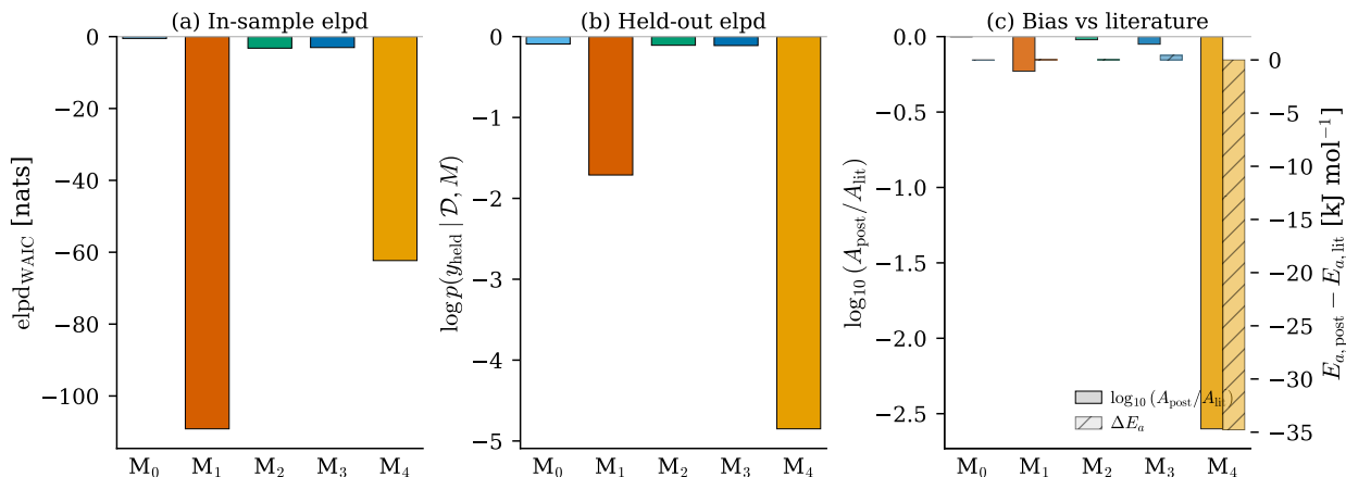
Figure 2: Comparator comparison on the multi-paper \text{Zn}^{2+} + e_s^- test problem. (a) In-sample predictive accuracy as \text{elpd}_{\text{WAIC}} ; higher is better. M_1 (naive pool) collapses to -109 nats; M_4 (weak prior) to -62 nats. (b) Out-of-sample predictive on the held-out Iwamatsu 550 °C point; same ordering. (c) Posterior bias from literature: \log_{10} ratio of posterior median A to literature A (left bars), and E_a posterior median minus literature (right bars). M_4 has -35 kJ/mol bias on E_a (unphysical negative Arrhenius slope).
