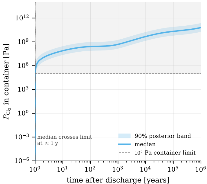
(a) Chloride fuel, no U buffer
