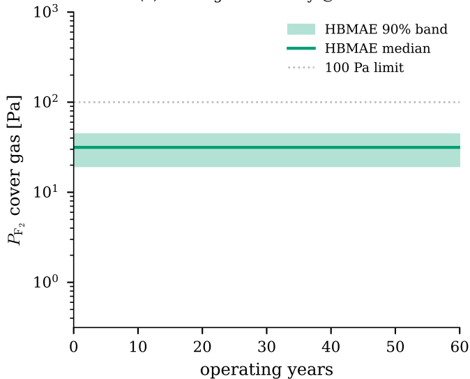
(a) Cover-gas inventory @ 600 °C
