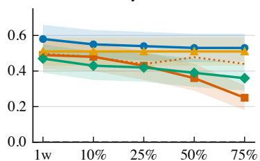
Anchor recovery
