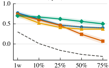
BERTScore (span)
