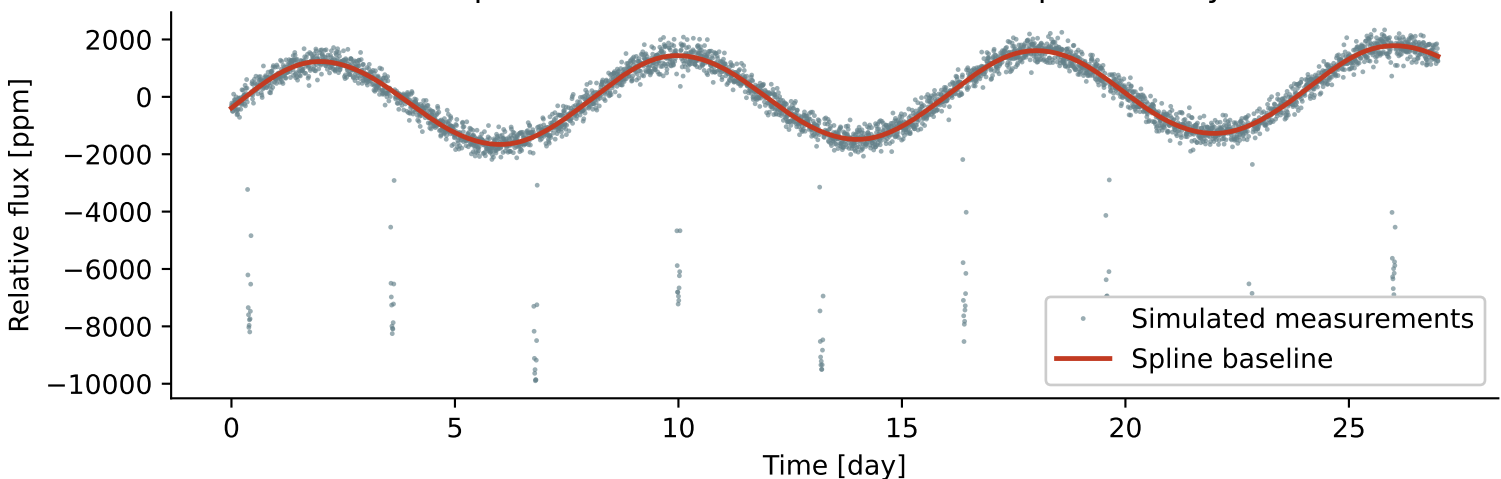
Intermediate: transit-masked spline detrending
