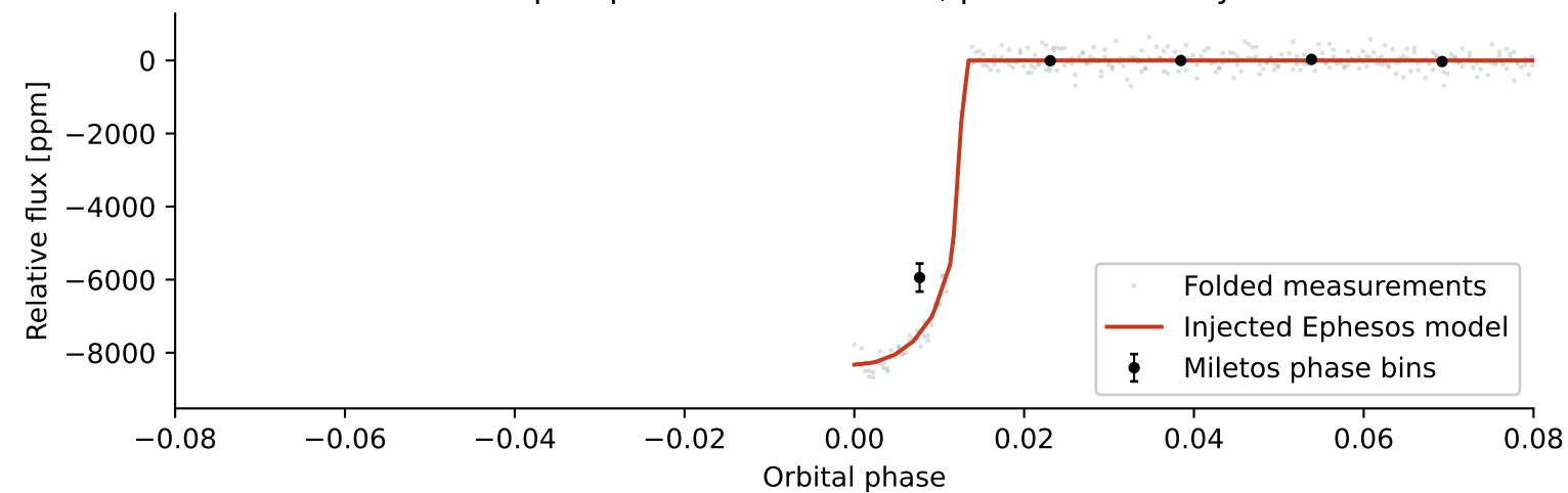
Output: phase-folded transit, period = 3.2 day
