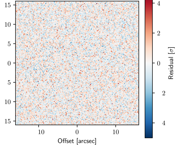
Poisson residual
