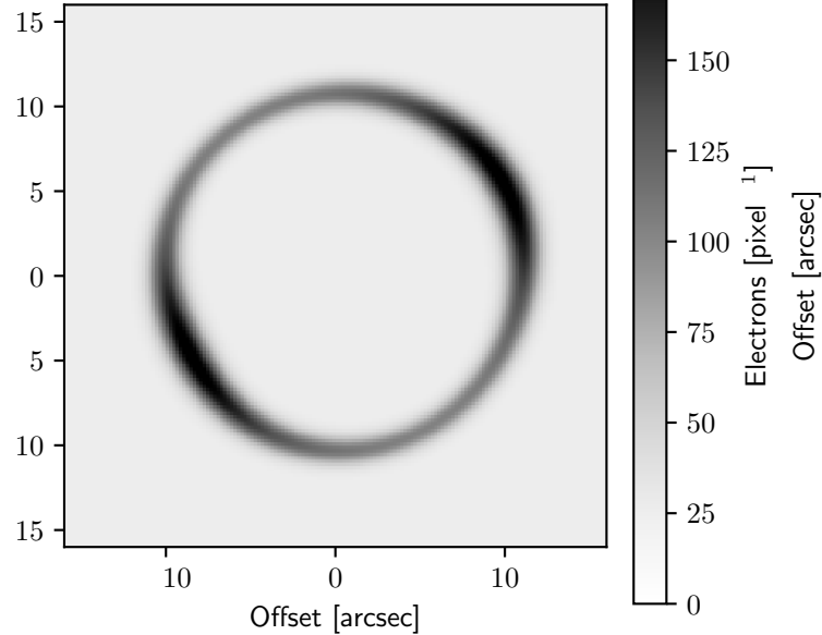
PCAT median model
