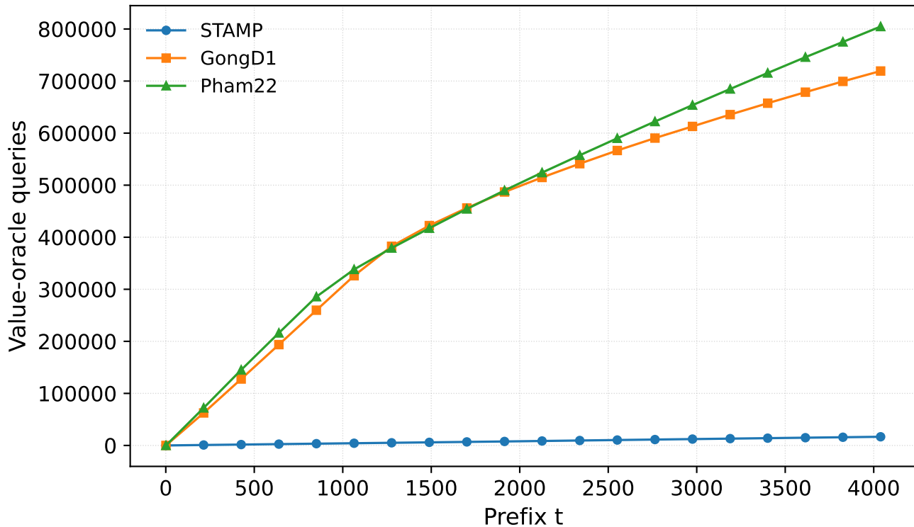
fb.bin (n=4039, K=3, B=807)
