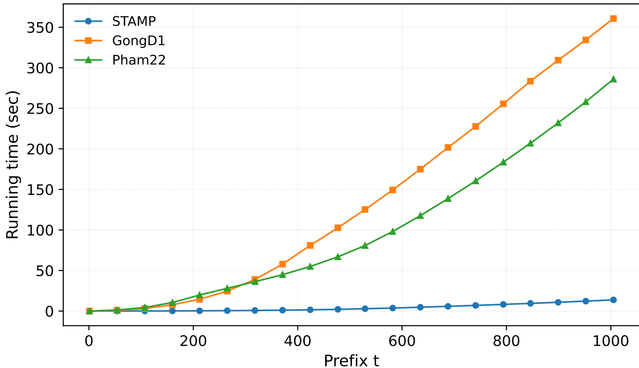
email.bin (n=1005, K=3, B=201)
