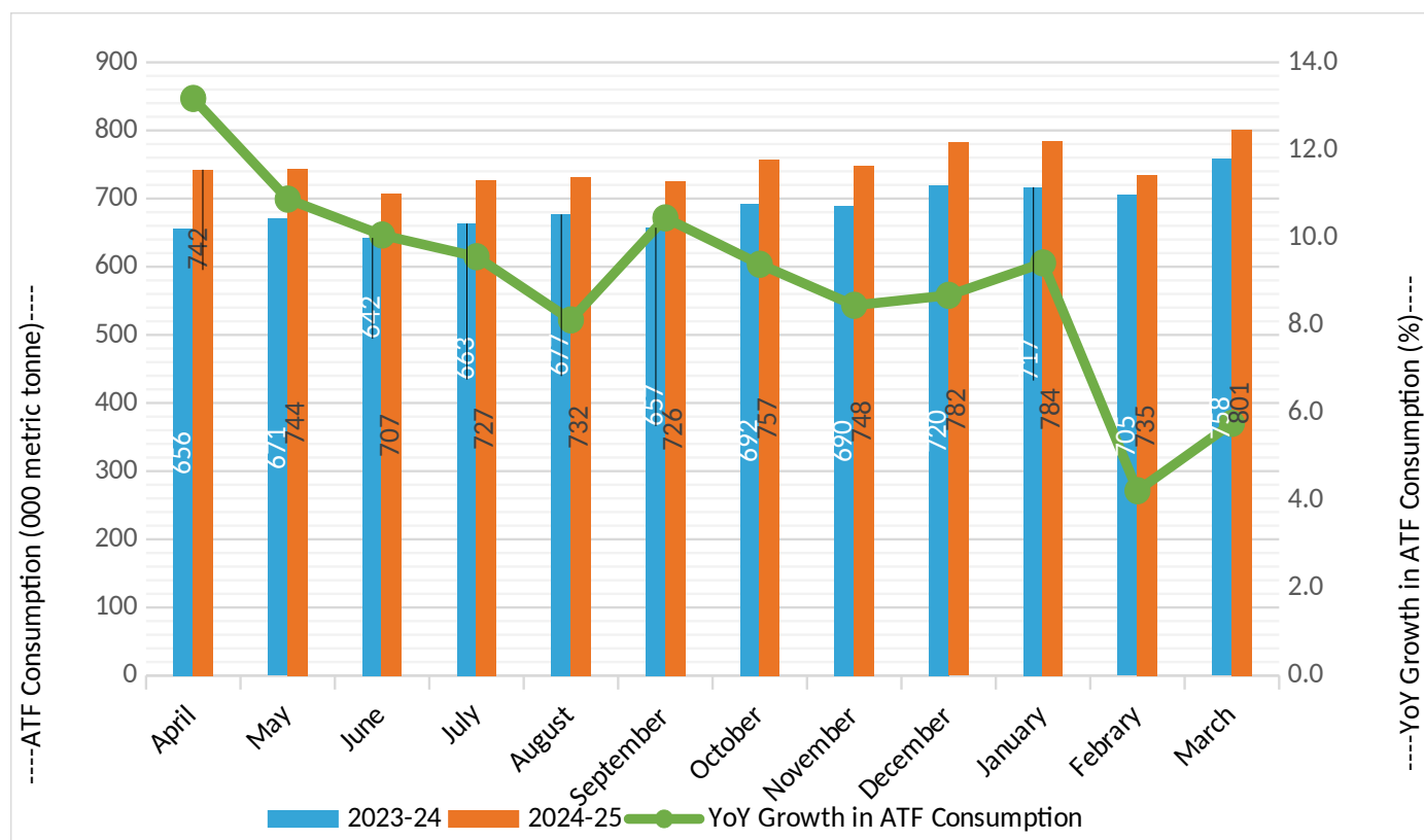
Chart 28: Year-on-Year growth of ATF consumption, 2024-25
