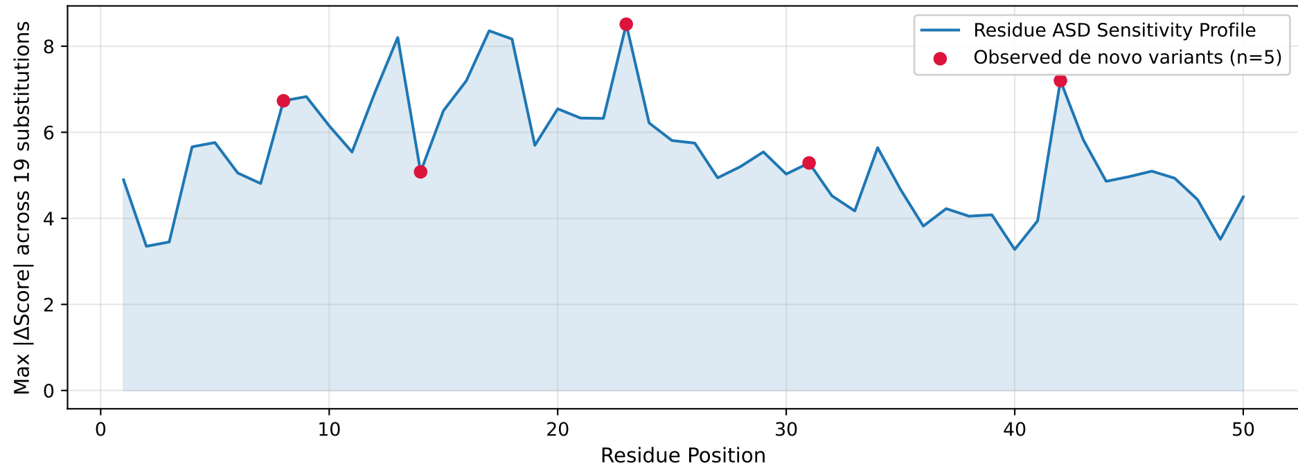
In-Silico Mutagenesis Profile: SHANK3
