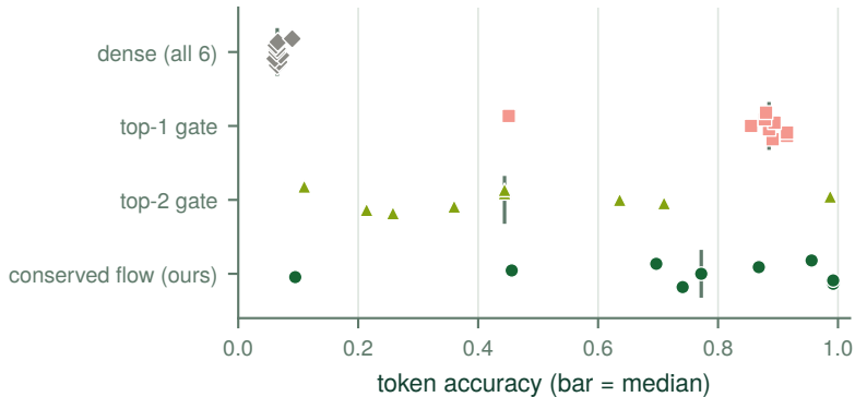
(a) accuracy, 9 seeds
