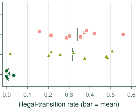
(b) illegal expert transitions
