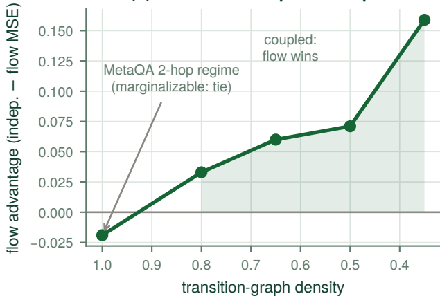
(b) flow wins iff steps are coupled
