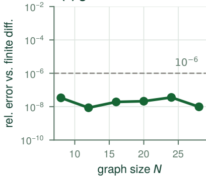
(a) gradient correctness
