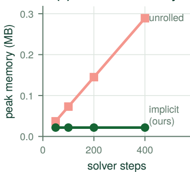
(b) backward memory
