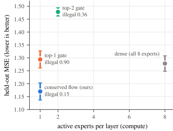
Figure 3: Conserved-flow routing is Pareto-dominant on the MoE accuracy/compute frontier (coupled regime, 3 seeds): lowest error at one active expert per layer, while the top- k gate needs more experts or routes illegally (illegal-transition rate annotated).
