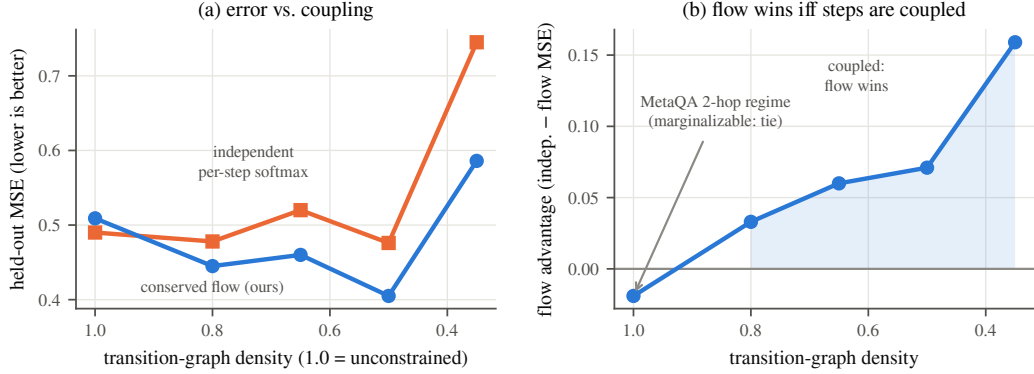
Figure 2: Conserved-flow routing beats independent per-step scoring exactly when reasoning steps are coupled. (a) held-out MSE vs. constraint density (left = more coupled); (b) the flow’s advantage crosses zero as the task becomes marginalizable. MetaQA 2-hop sits at the unconstrained end, predicting the tie we observe below.
