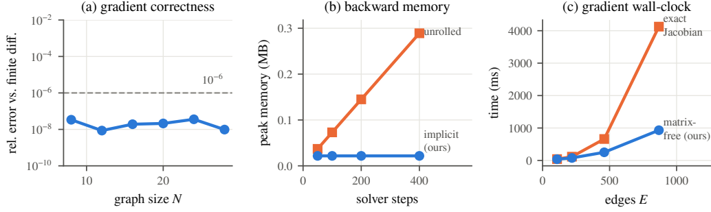
Figure 1: Differentiating and solving the flow at scale. (a) The implicit gradient matches a finite-difference gold standard to relative error \sim 10^{-8} across graph sizes. (b) Backward memory is flat in solver depth for implicit differentiation (forward runs under no_grad ) while unrolled autograd grows linearly. (c) The matrix-free (VJP-only) implicit gradient avoids the O(E^2) Jacobian, so its wall-clock scales far better with edges.
