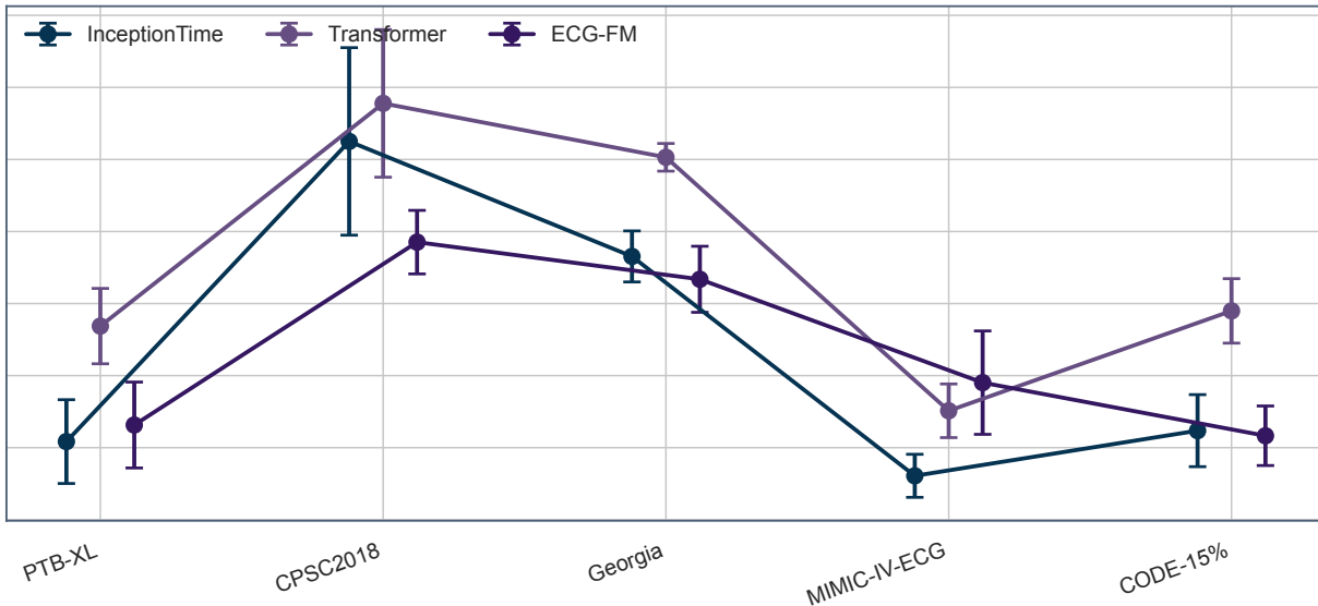
Uncertainty varies by target dataset
