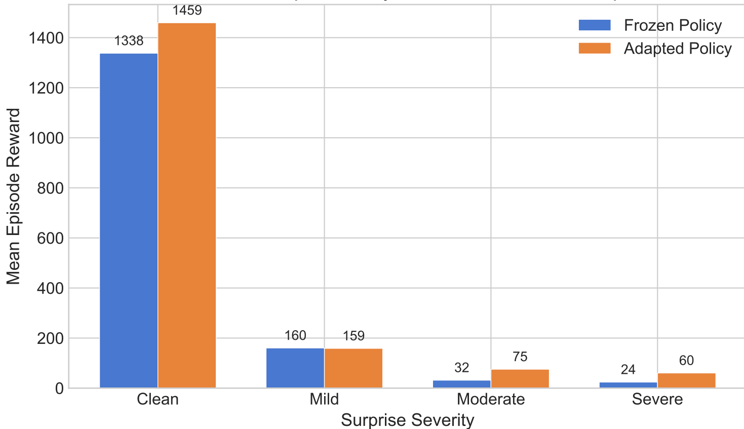
Frozen vs. Adapted Policy Performance Under Surprise
