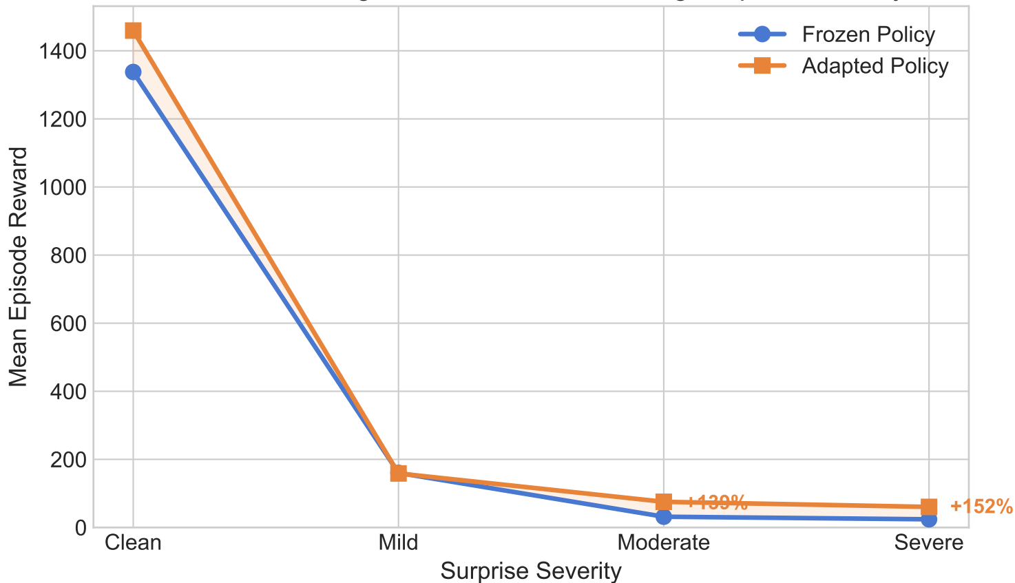
Performance Degradation Under Increasing Surprise Severity
