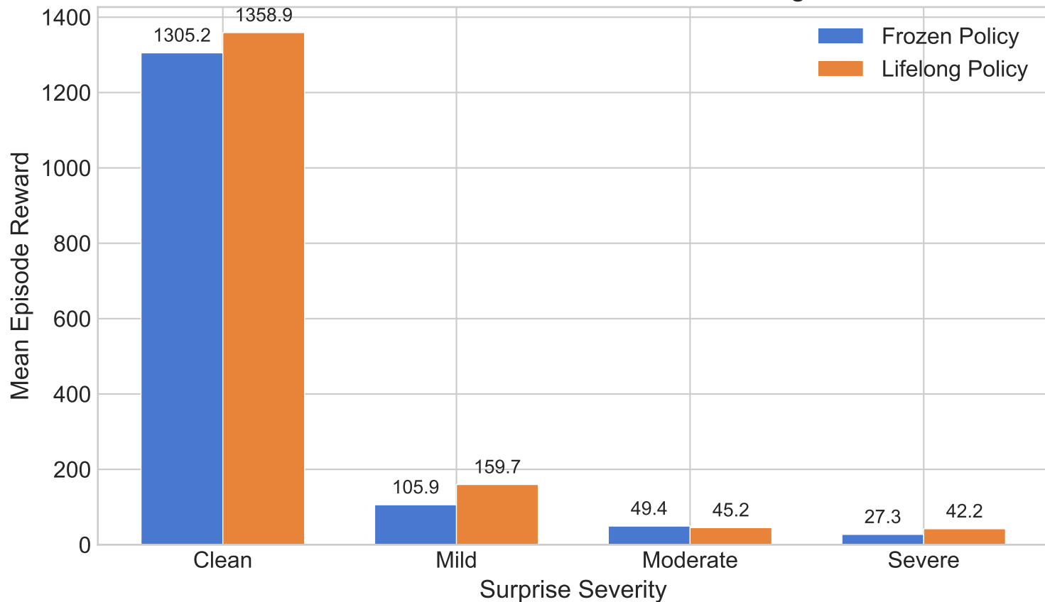
Saved Evaluation Results: Frozen vs Lifelong Reward
