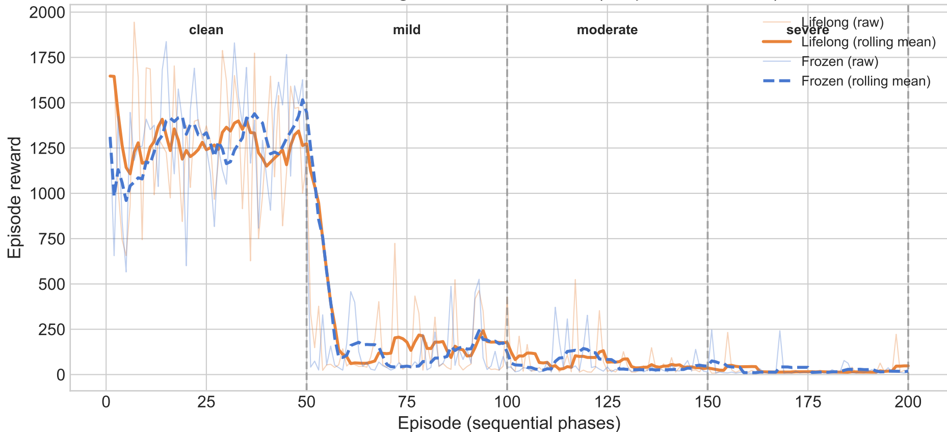
Continual Learning: Reward Over Time (Sequential Phases)
