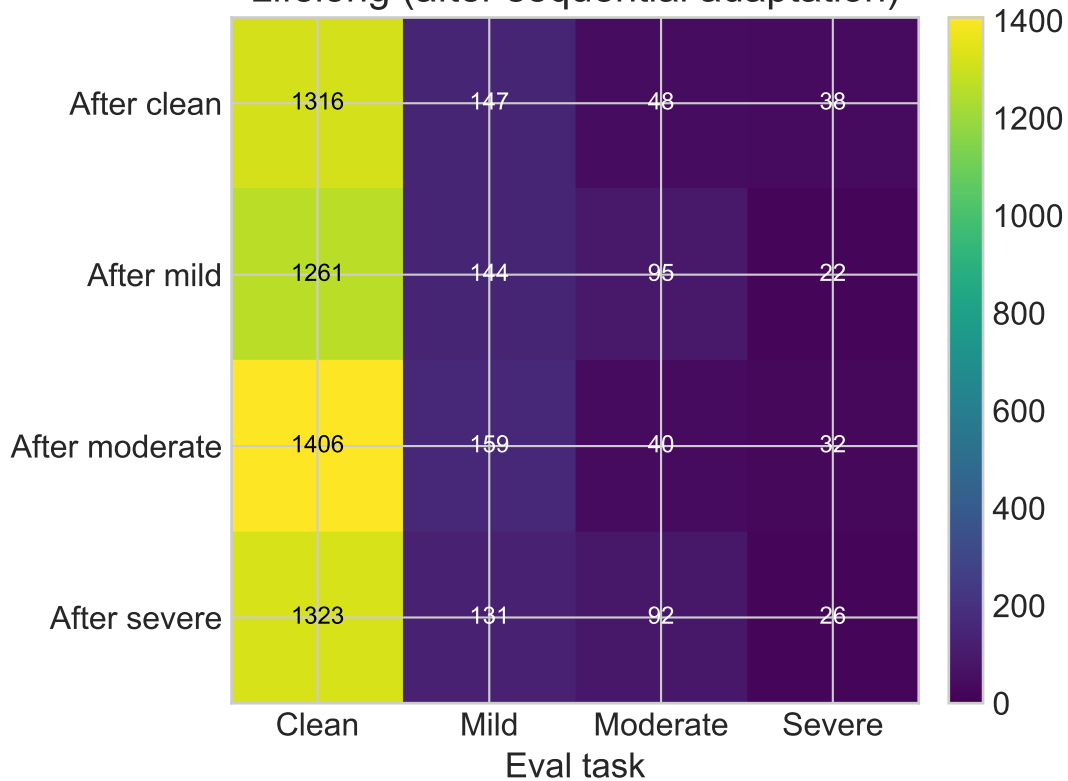
Lifelong (after sequential adaptation)
