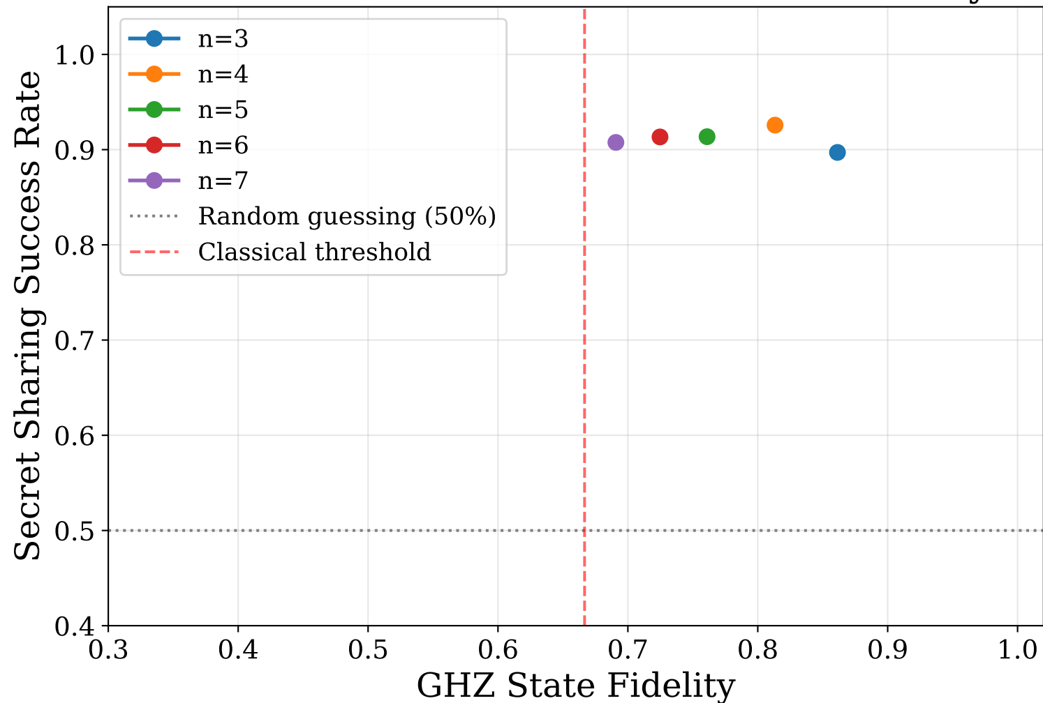
HBB Protocol Success Rate vs GHZ Fidelity
