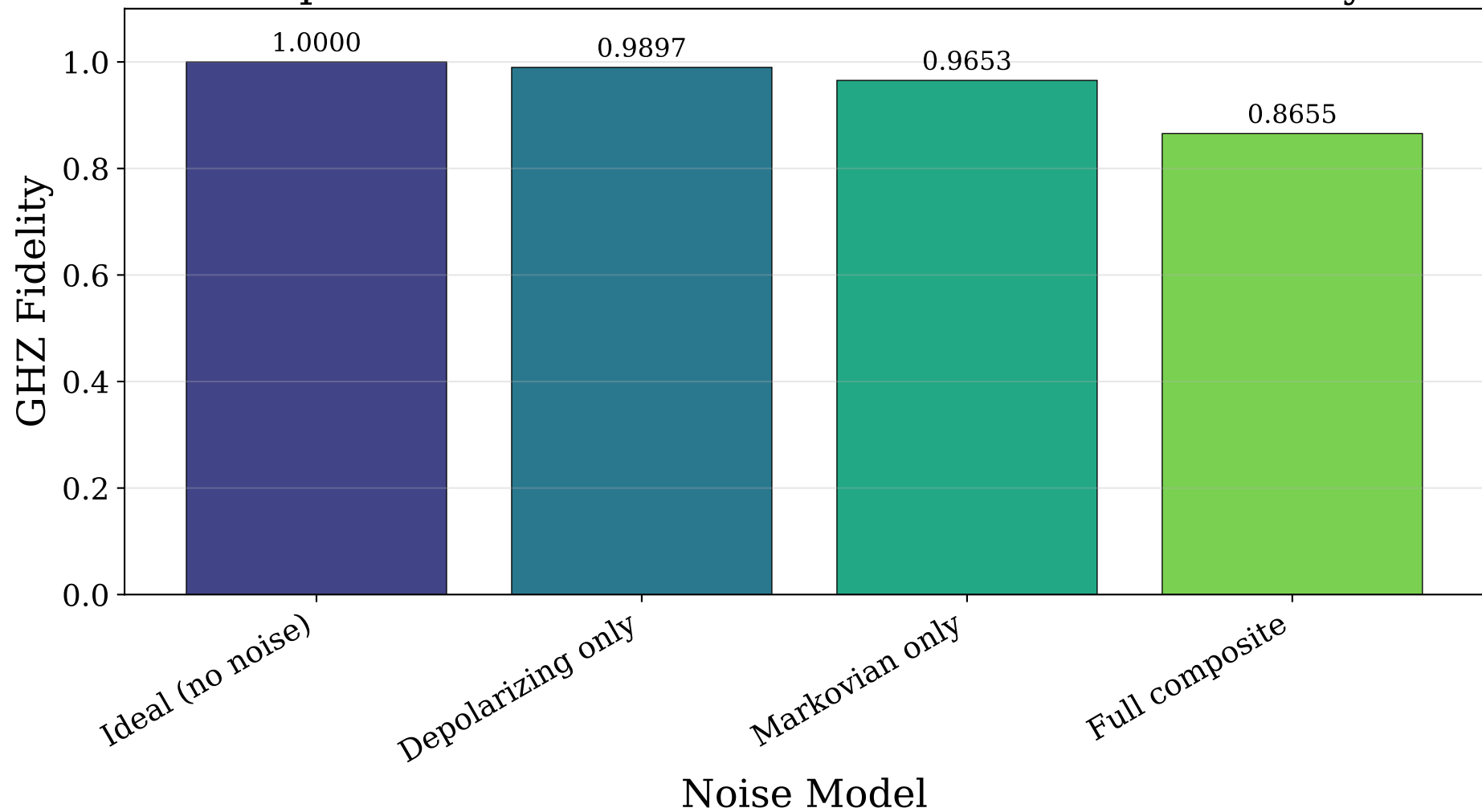
Impact of Individual Noise Sources on GHZ Fidelity
