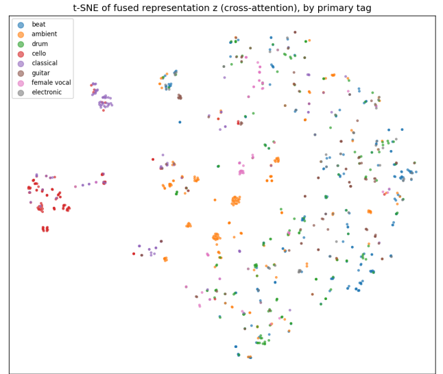
Figure 4: t-SNE of the fused representation z (cross-attention, 384-dim) over 1,500 held-out MagnaTagATune clips, coloured by primary tag. Broad timbral families separate — classical and vocal-led material occupy distinct regions — but the structure is diffuse rather than cleanly clustered, consistent with the modest Macro-F1 in Table 3.
