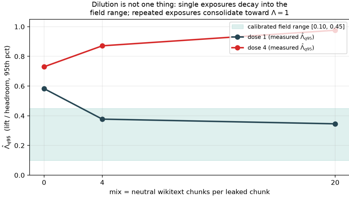
Figure 2: Corpus dilution is not one thing. Interleaving each leaked chunk with \text{mix} \in \{0, 4, 20\} neutral wikitext chunks holds per-item exposures fixed while total training grows. A single exposure (dose 1) decays into the calibrated field range [0.10, 0.45] ; repeated exposures (dose 4) consolidate toward complete memorization ( \Lambda = 0.98 ). Session-reproduction noise on \hat{\Lambda} is \leq 0.039 .
