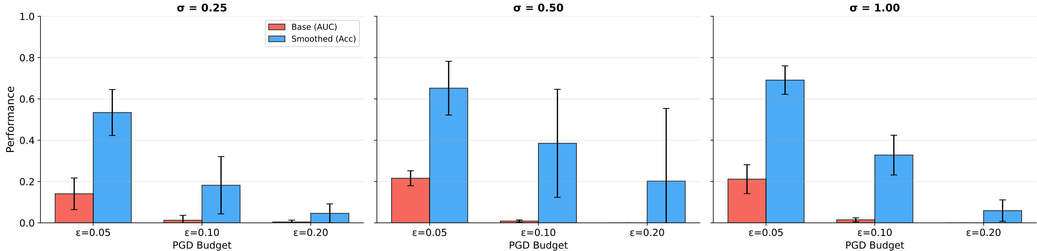
Base vs Smoothed Under PGD Attack (mean \pm std, 5 seeds)
