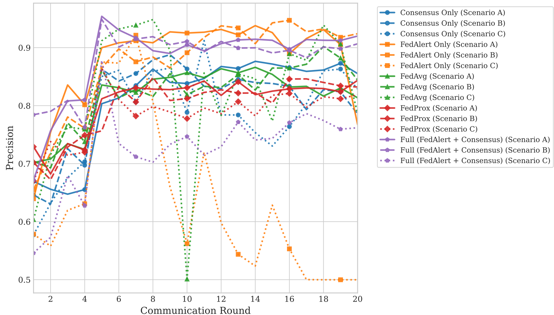
Precision vs. Communication Rounds
