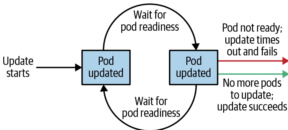
Figure 10-2. The Kubernetes Deployment life cycle
