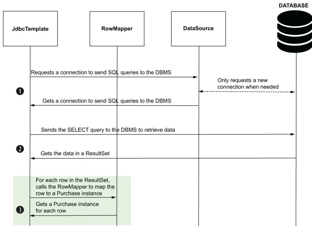
Figure 12.9 JdbcTemplate uses the RowMapper to change the ResultSet to a list of Purchase instances. For each row in the ResultSet , JdbcTemplate calls the RowMapper to map the row to a Purchase instance. The diagram presents all three steps JdbcTemplate follows to send the SELECT query: (1) get a DBMS connection, (2) send the query and retrieve the result, and (3) map the result to Purchase instances.
