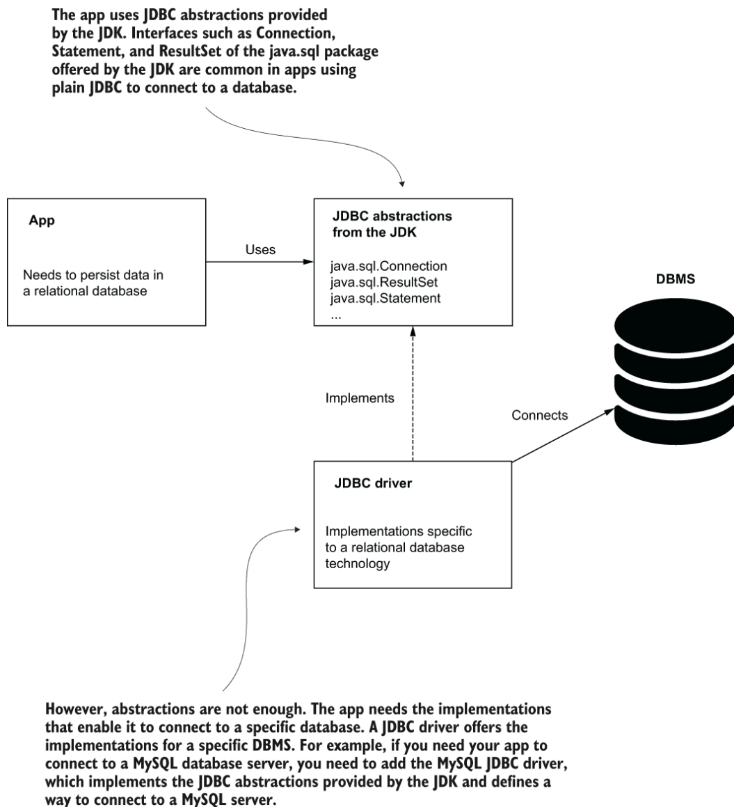
Figure 12.3 When connecting to a database, a Java app uses JDBC. The JDK provides a set of abstractions, but the app needs a certain implementation that depends on the relational database technology the app connects to. A runtime dependency named JDBC driver offers these implementations. For each specific technology, such a driver exists, and the app needs the exact driver that offers the implementations for the server technology it needs to connect to.
