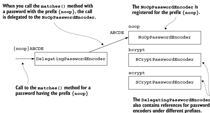
Figure 4.3 In this scenario, the DelegatingPasswordEncoder enlists a NoOpPasswordEncoder to handle passwords prefixed with {noop} , a BCryptPasswordEncoder for those beginning with {bcrypt} , and an SCryptPasswordEncoder for passwords starting with {sCrypt} . When a password is accompanied by the {noop} prefix, the DelegatingPasswordEncoder directs the task to the NoOpPasswordEncoder version.
