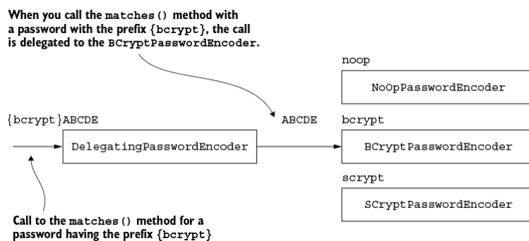
Figure 4.4 Here the DelegatingPasswordEncoder assigns the task of handling {noop} -prefixed passwords to the NoOpPasswordEncoder , {bcrypt} -prefixed passwords to the BCryptPasswordEncoder , and {sCrypt} -prefixed passwords to the SCryptPasswordEncoder . If a password carries the {bcrypt} prefix, the DelegatingPasswordEncoder routes the process to the BCryptPasswordEncoder 's mechanism.
