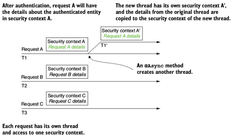
Figure 6.9 When using the MODE_INHERITABLETHREADLOCAL , the framework copies the security context details from the original thread of the request to the security context of the new thread.
