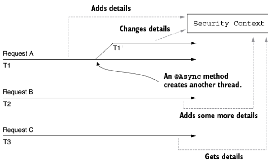
Figure 6.10 With MODE_GLOBAL used as the security context management strategy, all the threads access the same security context. This implies that these all have access to the same data and can change that information. Because of this, race conditions can occur, and you must take care of synchronization.
