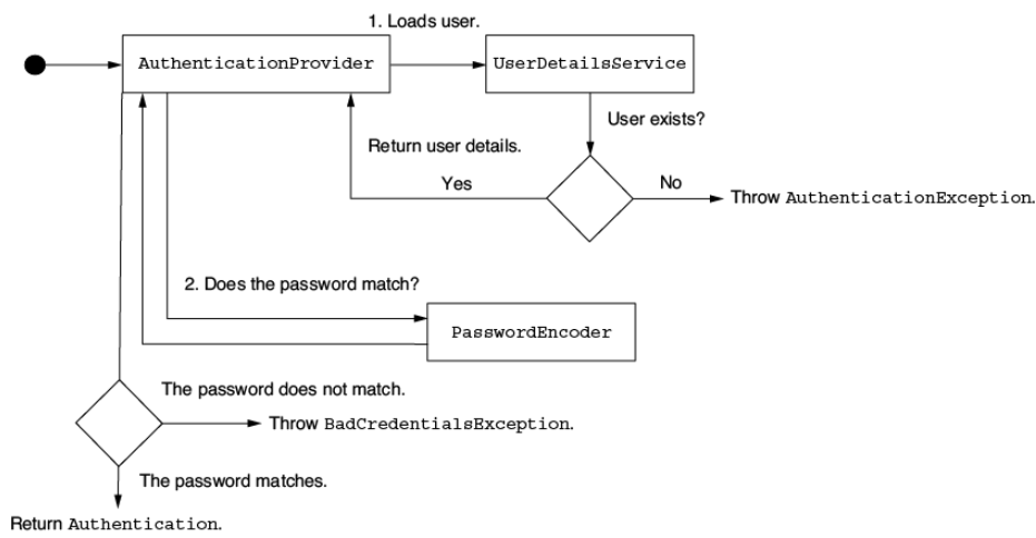
Figure 6.6 The AuthenticationProvider enacts a tailored authentication procedure. It confirms the authentication request by retrieving user details through a specific UserDetailsService implementation, and it validates the password using a PasswordEncoder if the password is correct. If the user is not found or the password is inaccurate, the AuthenticationProvider will raise an AuthenticationException .
