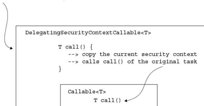
Figure 6.11 DelegatingSecurityContextCallable is designed as a decorator of the Callable object. When building such an object, you provide the callable task that the application executes asynchronously. DelegatingSecurityContextCallable copies the details from the security context to the new thread and then executes the task.
