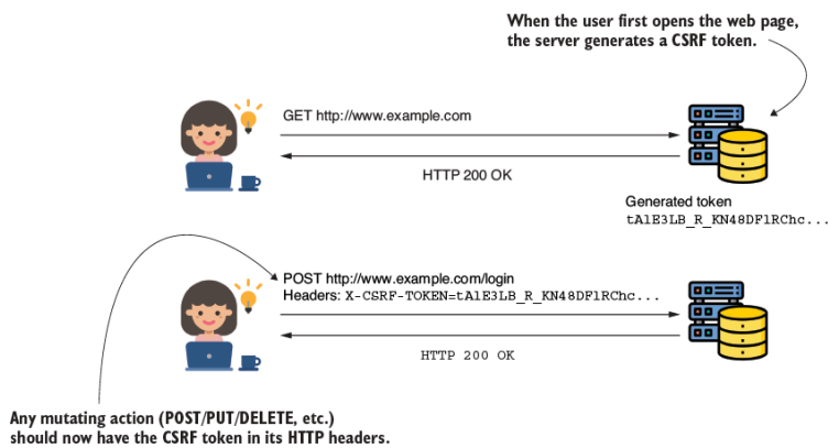
Figure 9.2 To make a POST request, the client needs to add a header containing the CSRF token. The application generates a CSRF token when the page is loaded (via a GET request), and the token is added to all requests that can be made from the loaded page. This way, only the loaded page can make mutating requests.
