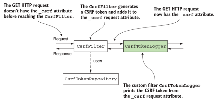
Figure 9.4 Inserting the CsrfTokenLogger (highlighted) following the CsrfFilter allows it to retrieve the token's value from the request's _csrf attribute, which is where the CsrfFilter deposits it. The CsrfTokenLogger outputs the CSRF token onto the application's console, from where it can be retrieved for use in making an HTTP POST request to an endpoint.
