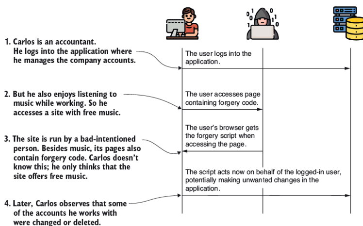
Figure 9.1 After the user logs into their account, they access a page containing forgery code. This code impersonates the user and can execute unwanted actions on behalf of the user.
