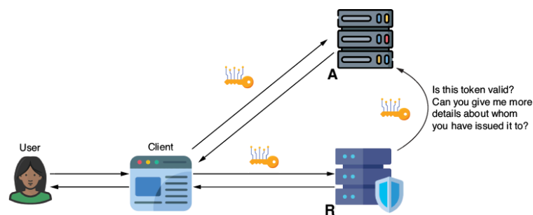
Figure 15.6 Token introspection. In situations where the resource server cannot depend on signature-based validation of access tokens (such as when token revocation is necessary), or when the token does not contain detailed information (as with opaque tokens), the resource server is required to make inquiries to the authorization server. This is done to ascertain the validity of a token and to gather additional information about it.
