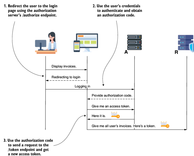
Figure 15.3 The authorization code grant type. The client redirects the user to the authorization server's login page. After the user successfully authenticates, the authorization server redirects back to the client, providing an authorization code. The client uses the authorization code to obtain an access token.
