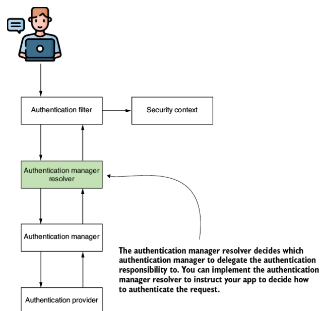
Figure 15.8 Implementing an authentication manager resolver, you tell your app which authentication manager to delegate the authentication responsibility to.
