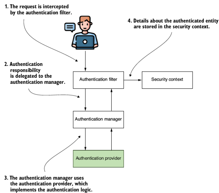
Figure 15.7 The authentication class design. During the authentication procedure, the filter captures the request and passes it on to an authentication manager component. This manager then employs an authentication provider that executes the necessary authentication logic. Upon successful authentication, the application records the authenticated principal's details in the security context.
