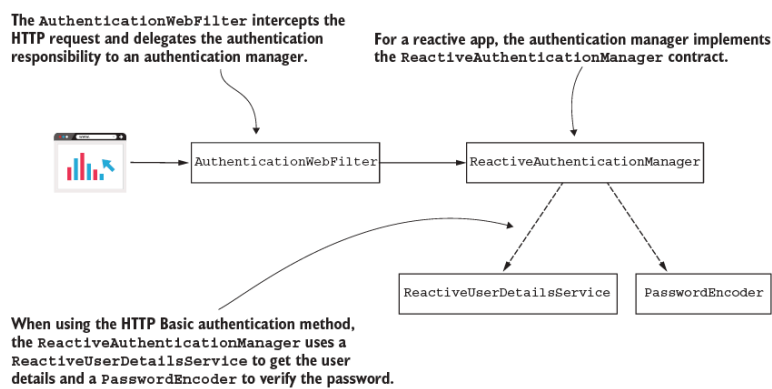
Figure 17.5 An AuthenticationWebFilter intercepts the request and delegates the authentication responsibility to a ReactiveAuthenticationManager . If the authentication logic involves users and passwords, the ReactiveAuthenticationManager uses a ReactiveUserDetailsService to find the user details and a PasswordEncoder to verify the password.
