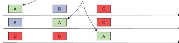
Figure 17.3 In the figure, each arrow represents the timeline of a different thread, and squares represent the processed tasks from requests A, B, and C. Because in a reactive app, tasks from one request might be handled on multiple threads, the authentication details cannot be stored at the thread level anymore.
