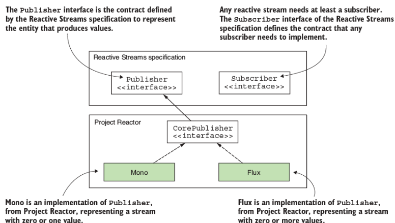
Figure 17.2 In a reactive stream, a publisher produces values, and a subscriber consumes them. Contracts defined by the Reactive Streams specification describe publishers and subscribers. Project Reactor implements the Reactive Streams specification and implements the Publisher and Subscriber contracts. In the figure, the components we use in the examples in this chapter are shaded.
