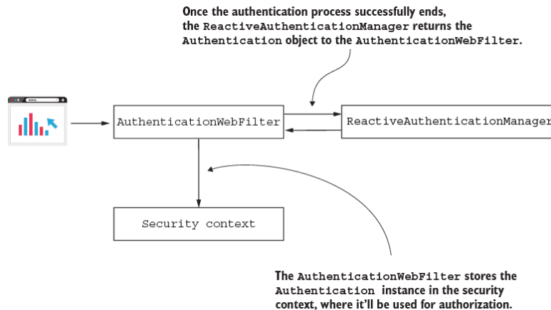
Figure 17.6 Once the ReactiveAuthenticationManager successfully authenticates the request, it returns the Authentication object to the filter. The filter stores the Authentication instance in the SecurityContext .
