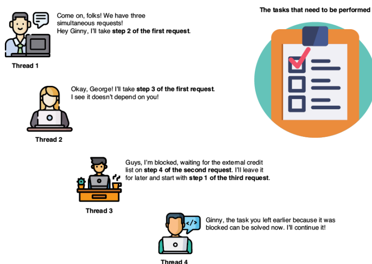
Figure 17.4 An analogy of the way a reactive app works. A thread doesn't take a request's tasks in order and wait when it's blocked. Instead, all tasks from all requests are on a backlog. Any available thread can work on tasks from any request. This way, independent tasks can be solved in parallel, and the threads don't stay idle.
