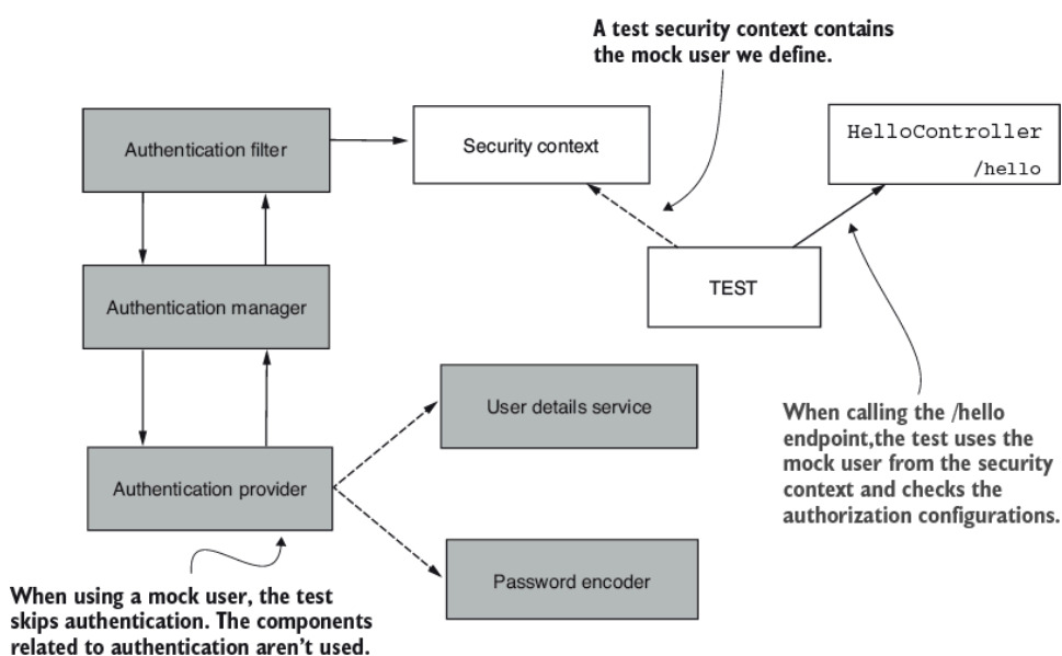
Figure 18.4 When running the test, we skip authentication. The test uses a mock SecurityContext and calls the /hello endpoint exposed by HelloController. We add a mock user in the test SecurityContext to verify that the behavior is correct according to the authorization rules. If we don't define a mock user, we expect the app to not authorize the call, but if we define a user, we expect that the call succeeds.
