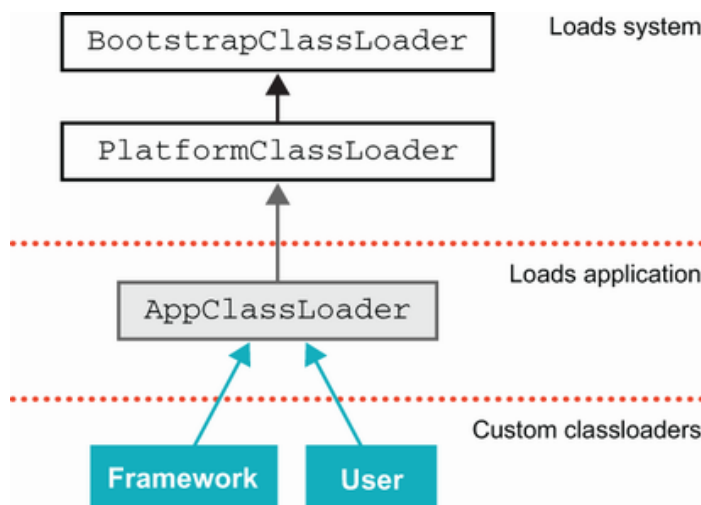
Figure 4.3 Classloader hierarchy
