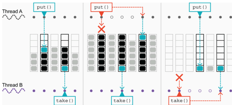
Figure 6.5 The BlockingQueue
