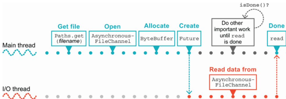
Figure 6.9 Using Future in Java
