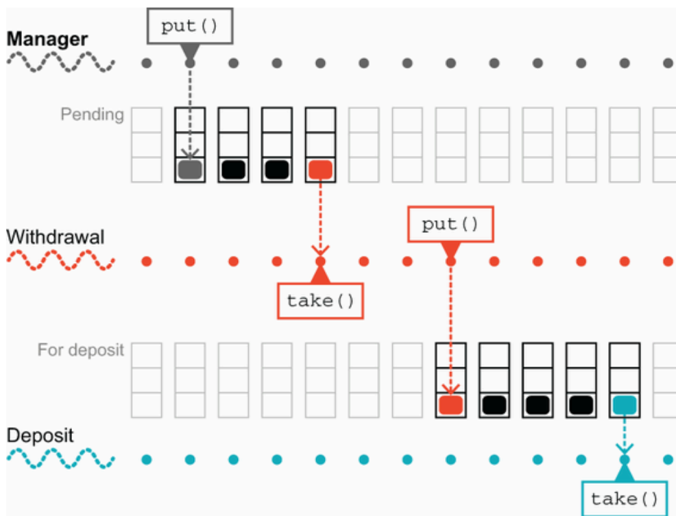
Figure 6.6 Handling accounts with queues
