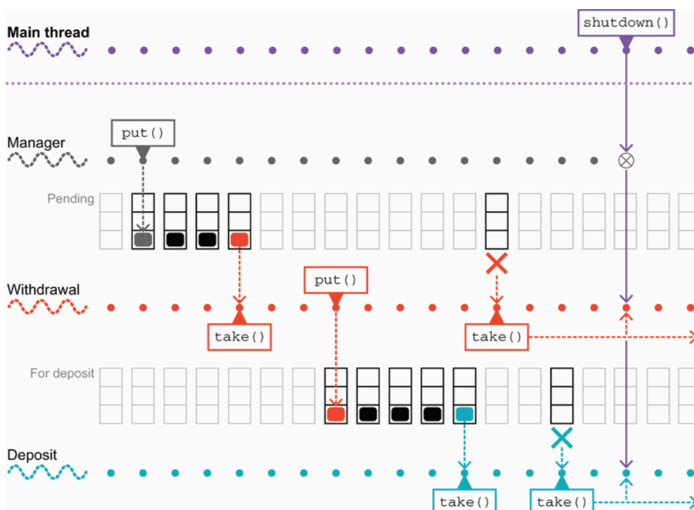
Figure 6.7 An incorrect shutdown sequence
