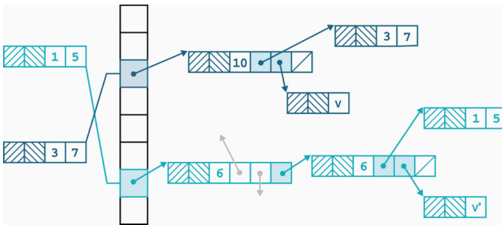
Figure 6.2 The classic view of a HashMap
