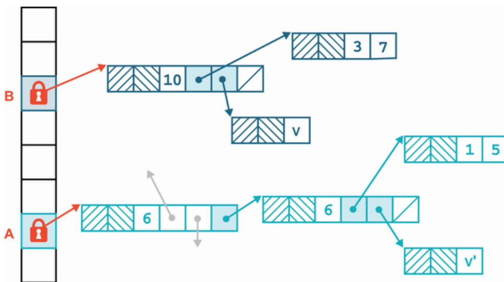
Figure 6.3 Lock striping
