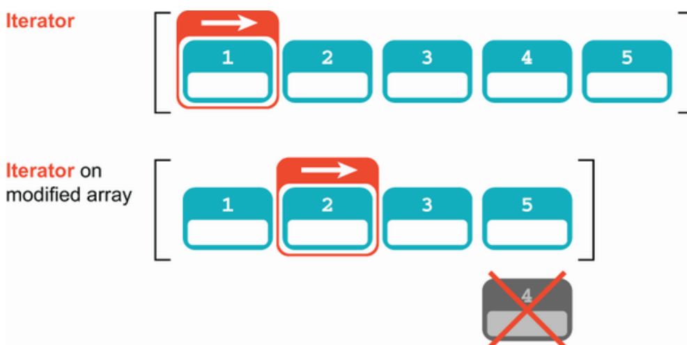
Figure 6.4 Copy-on-write array
