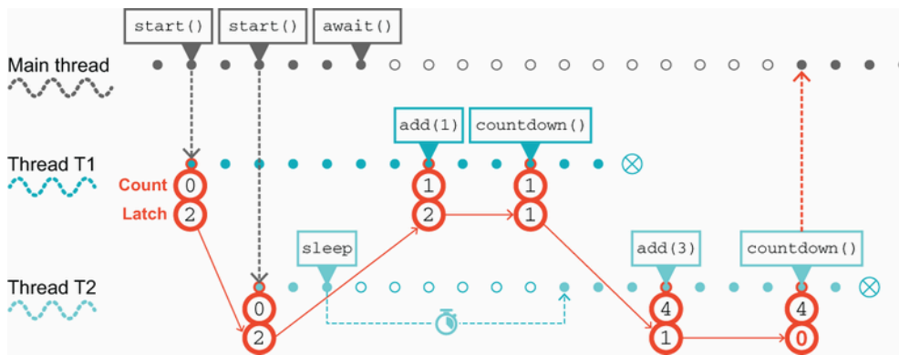
Figure 6.1 Using a CountDownLatch
