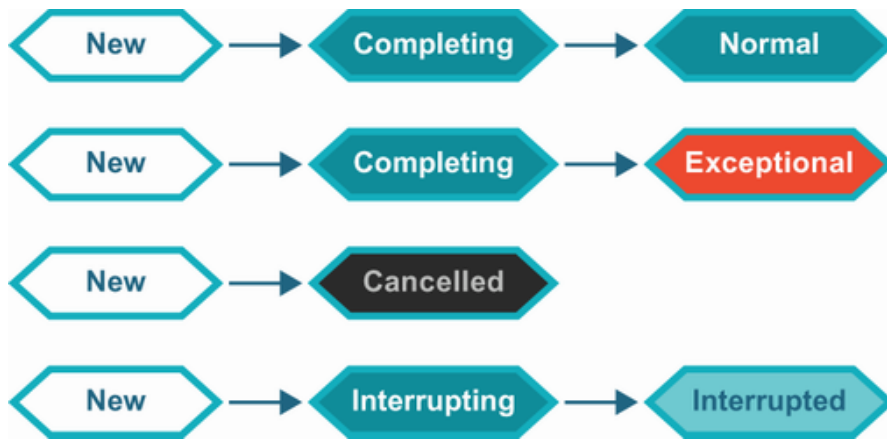
Figure 6.10 State model for tasks
