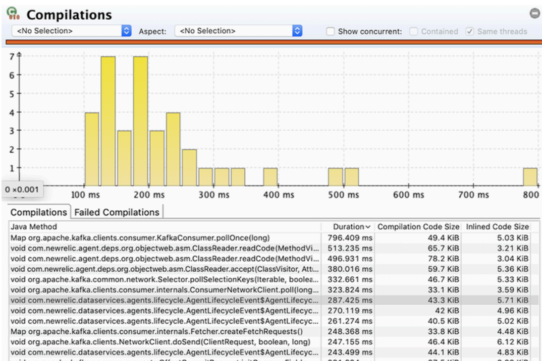
Figure 7.11 JMC JIT compilation
