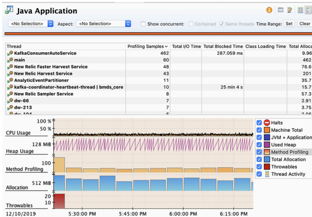
Figure 7.8 JMC dashboard
