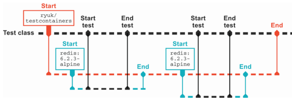
Figure 14.2 Fields and @Container
