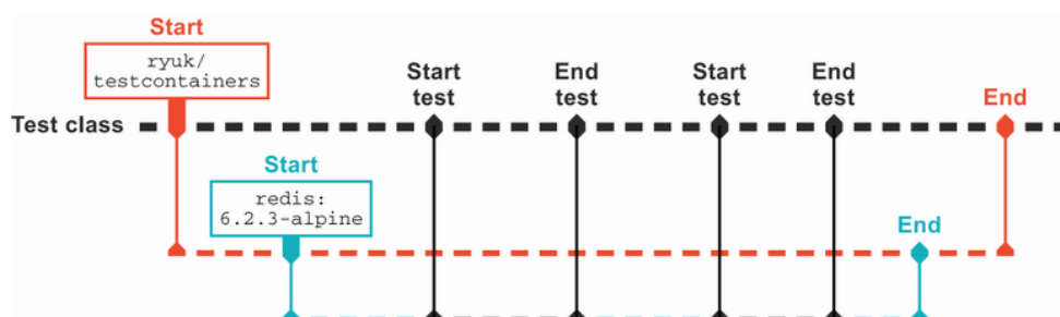
Figure 14.1 Testcontainers execution
