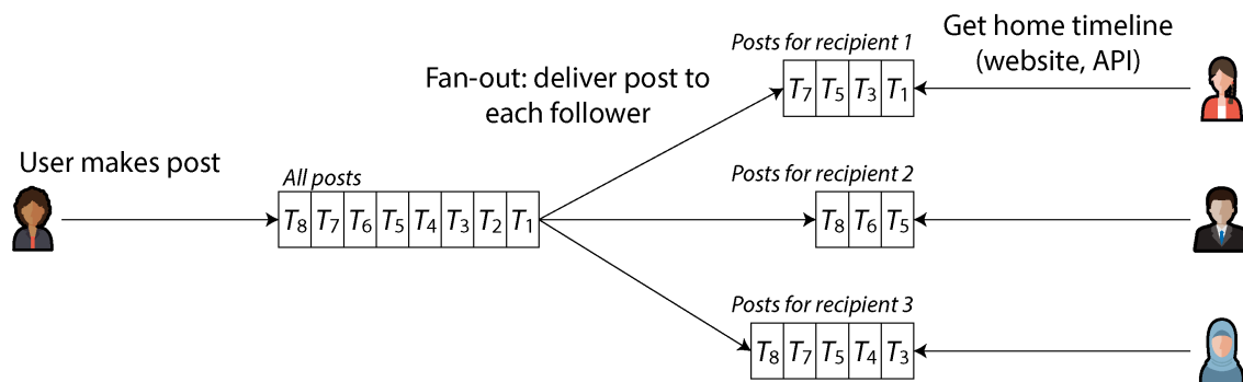
Figure 2-2. Fan-out: delivering new posts to every follower of the user who made the post
