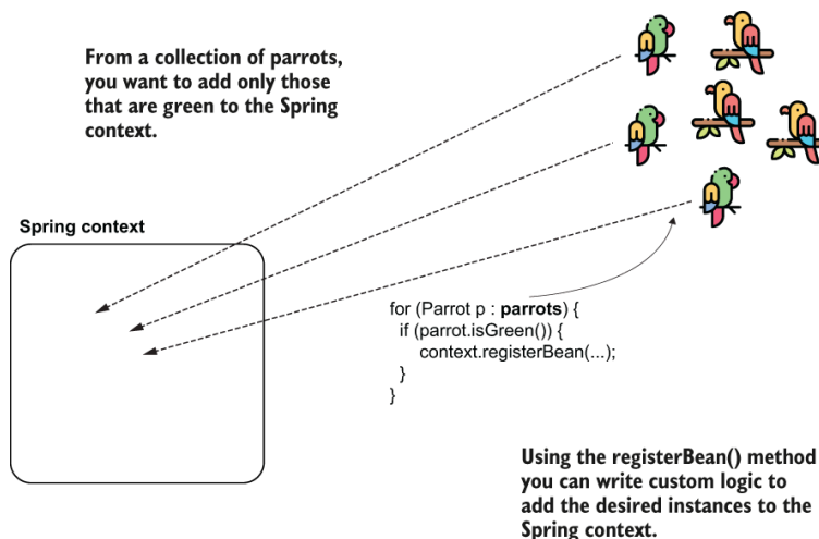
Figure 2.13 Using the registerBean() method to add specific object instances to the Spring context
