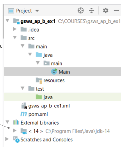
Figure 2.5 With a default pom.xml file, your project only uses the JDK as an external dependency. One of the reasons you change the pom.xml file (and the one we'll use in this book) is to add new dependencies your app needs.
